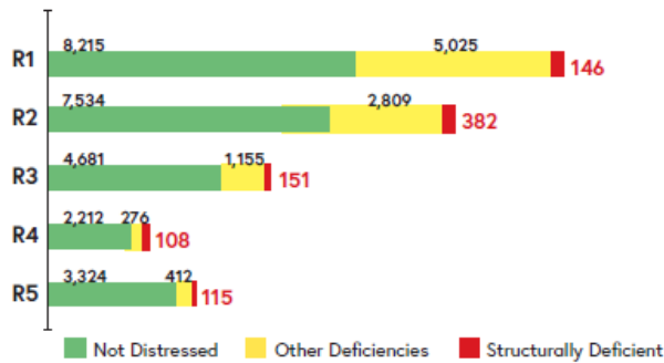
ODOT bridge conditions by 1,000 square feet of deck. Note that Region 1, which includes the Portland Metro area, includes the greatest quantity by bridge deck area.
