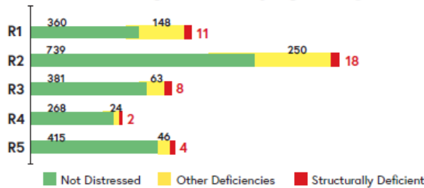
ODOT bridge conditions by count.
